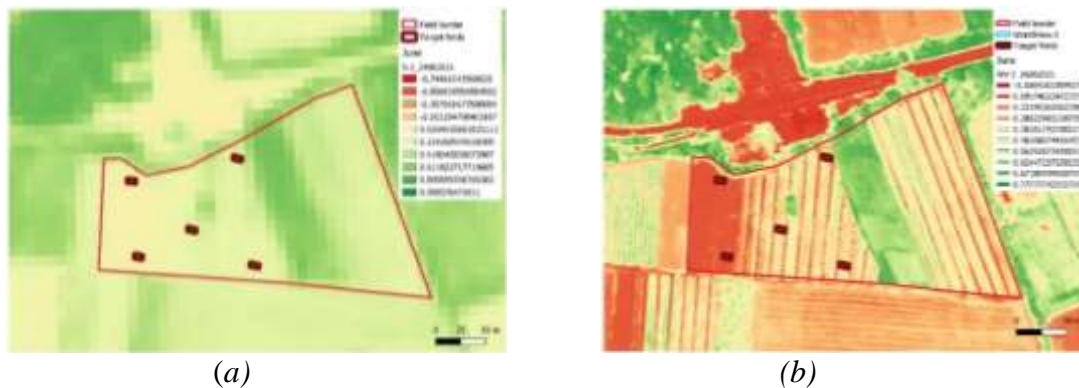
Figure 3. NDVI values: WorldView-3 (a) and Sentinel-2 (b)
