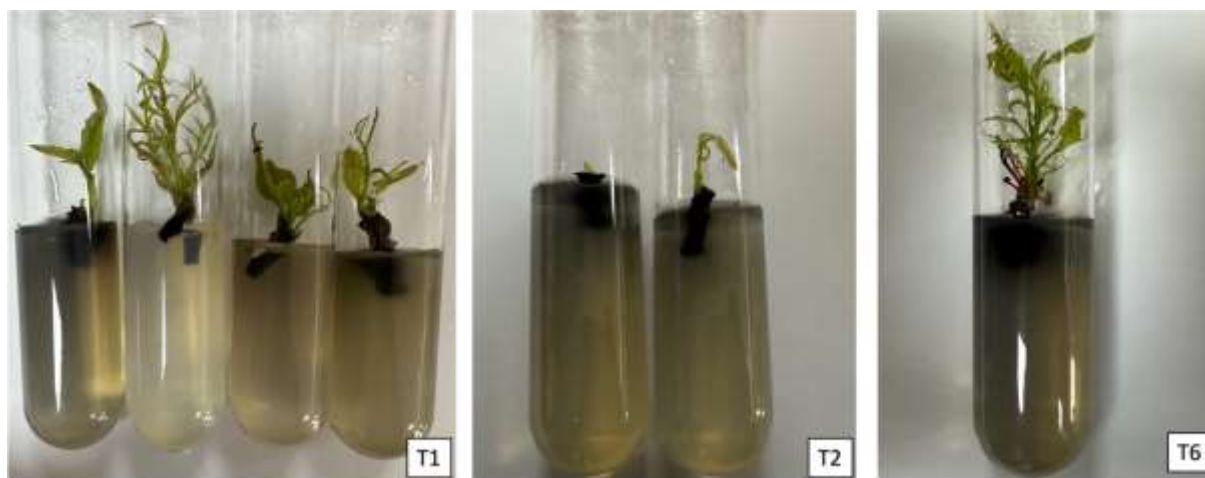
Figure 2. Shoot development in applied explants. T1: 5% NaOCl, T2: 10% NaOCl and T6: HOCl.
