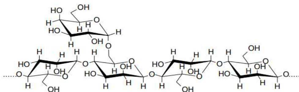
Figure 2. Galactomannan structure
